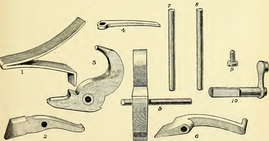
Lock-work of the Anson and Decey Hammerless Gun.
